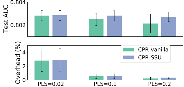
Figure 9. CPR trades off performance and accuracy.
